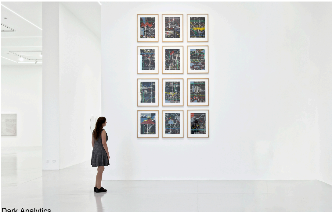
Dark Analytics
