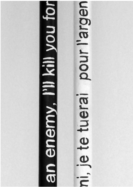
Obstacles, Coma
